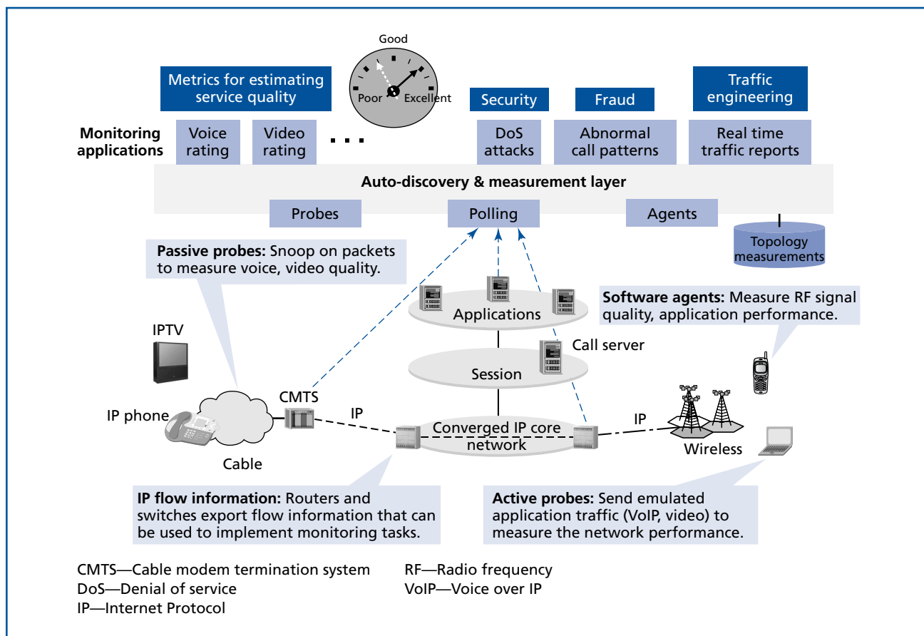
Figure 1. Monitoring infrastructure for next generation converged networks.
